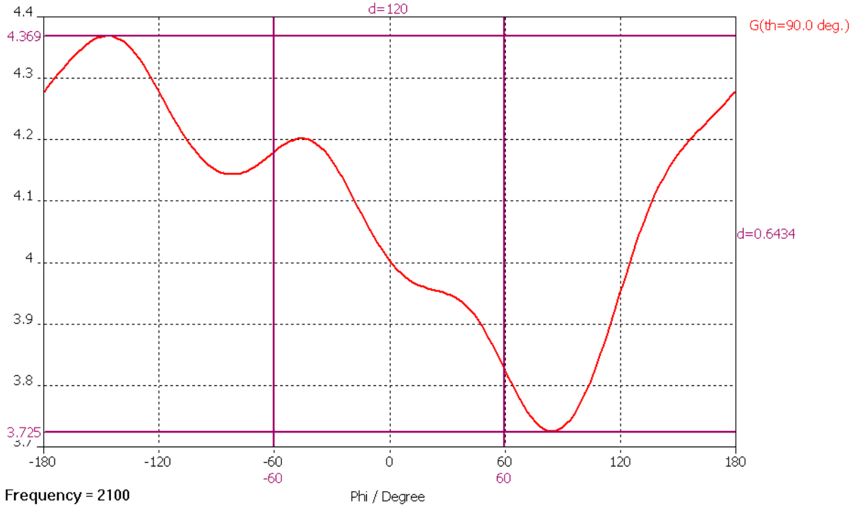
Farfield farfield (f=2100) [1] Gain_Abs in dB
